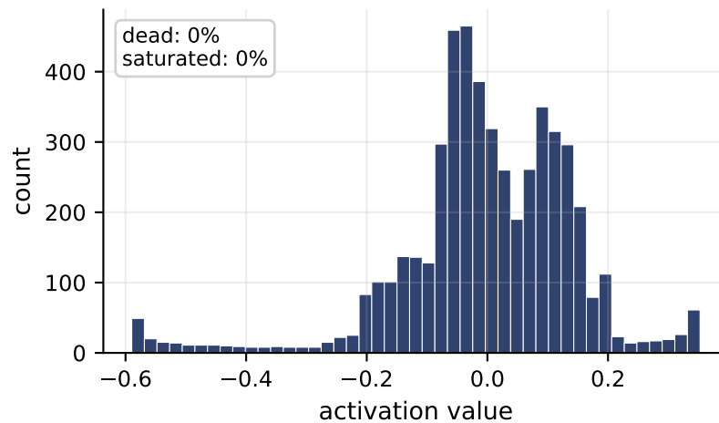
L4 (20 neurons)
